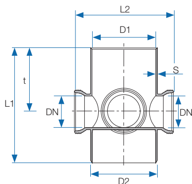
Floor collector outlet 100 + outlet 110
