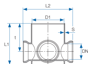
Floor collector with vertical outlet 50/130
