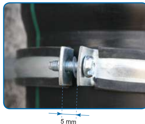
Figure 6 - Correct tightening:
