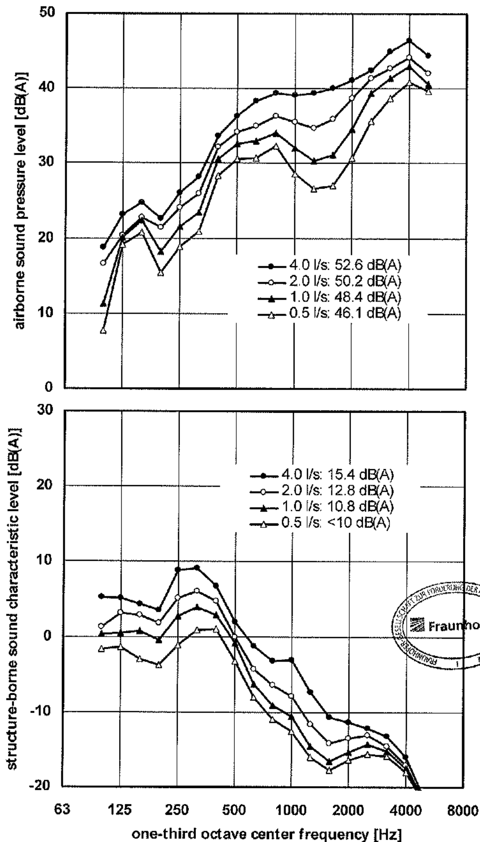
Figure 2 Wastewater pipe system "Ultra Silent+ 110 x 4.8" mounted according to figure 4, using pipe clamps "Müpro yellow, with spacer 5 mm". Airborne sound pressure level (above) and structure-borne sound characteristic level (below) measured at various flow rates according to DIN EN 14366.
