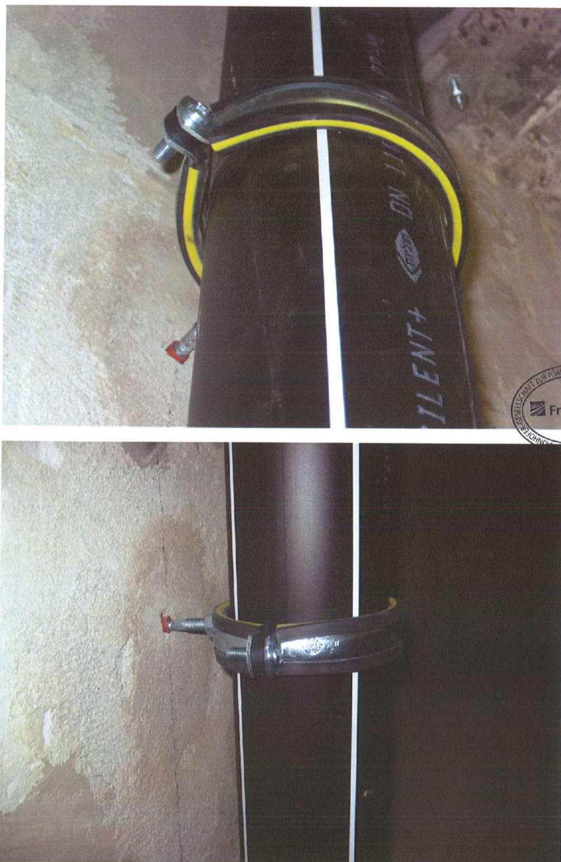
Figure 5 Waste water system "Ultra Silent+ 110 x 4.8" with pipe clamps "Müpro yellow, with spacer 5 mm".
