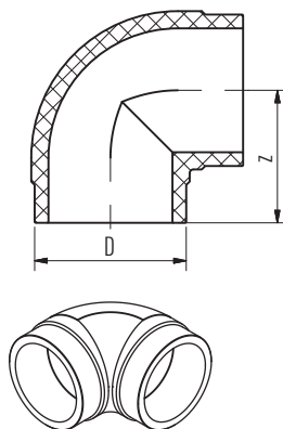
Injection molded fitting
